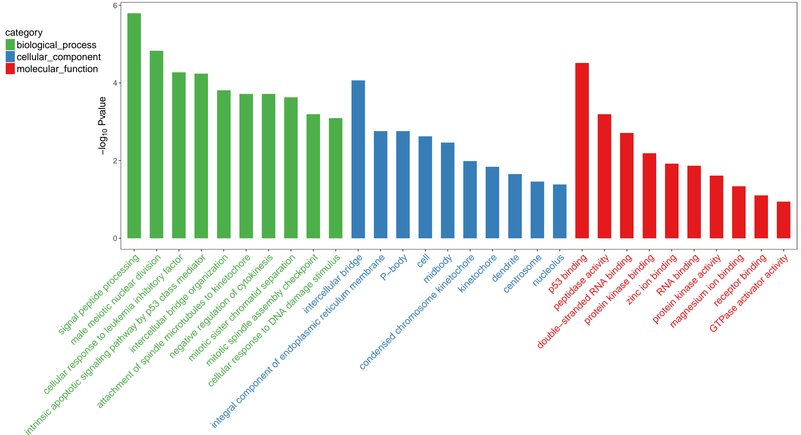
E120-vs-D0(Total): Top 30 GO Term
