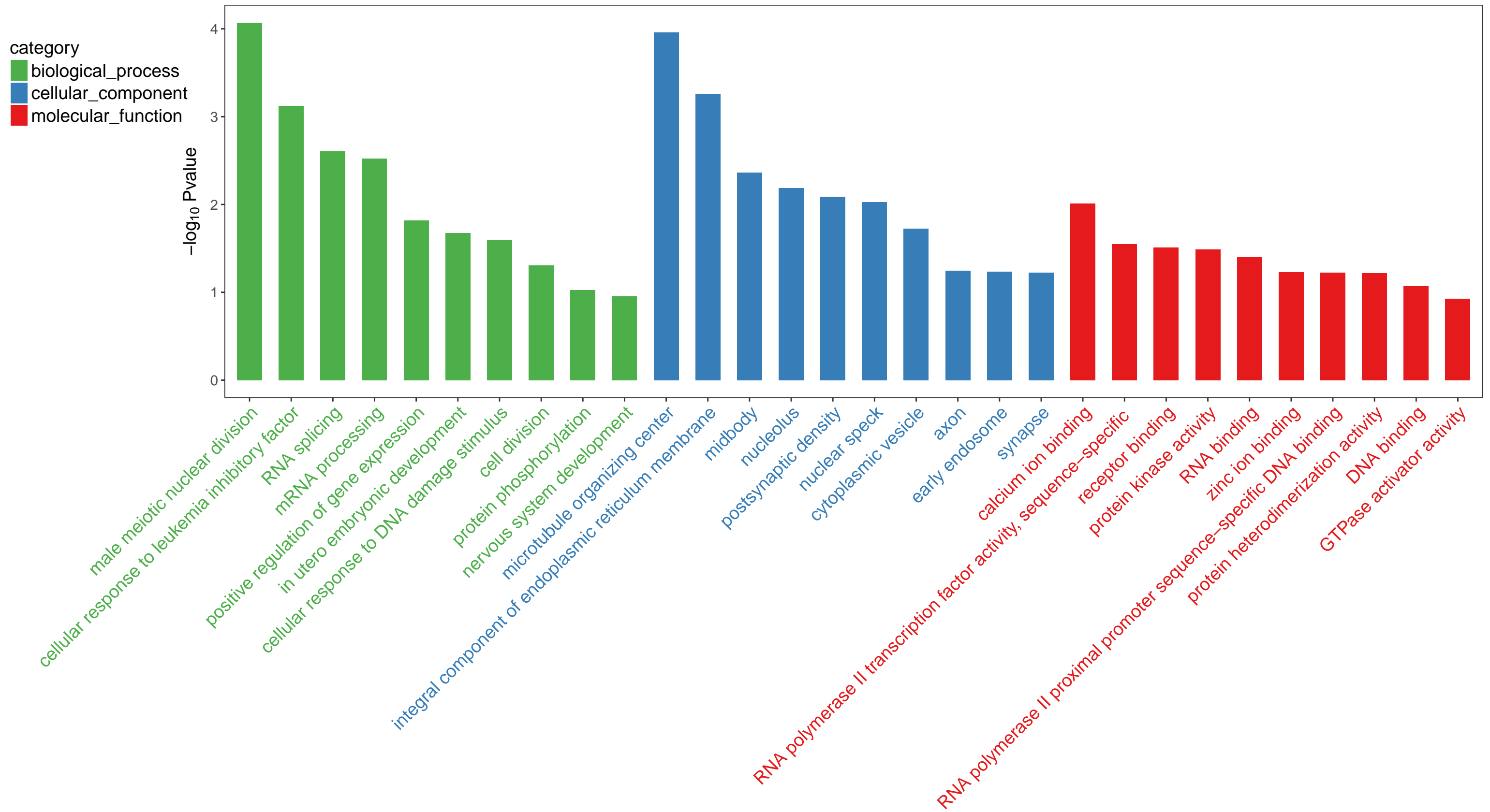
D0-vs-D360(Total): Top 30 GO Term
