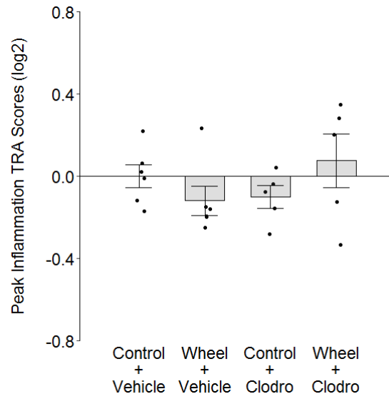
Supplementary Figure 3. TRA composite scores in the immunocompetent C57BL/6-EO771 model of breast cancer as a function of voluntary wheel running x clodronate treatment at Day 1 for peak inflammation from Kong et al. (2020) (genes up-regulated by 50% at peak inflammation vs. baseline, before subsequent resolution of inflammation) (Supplementary Data 6). Mean \pm SEM and individual data points, with n = 5-6 mice per group. Clodro: Clodronate.
