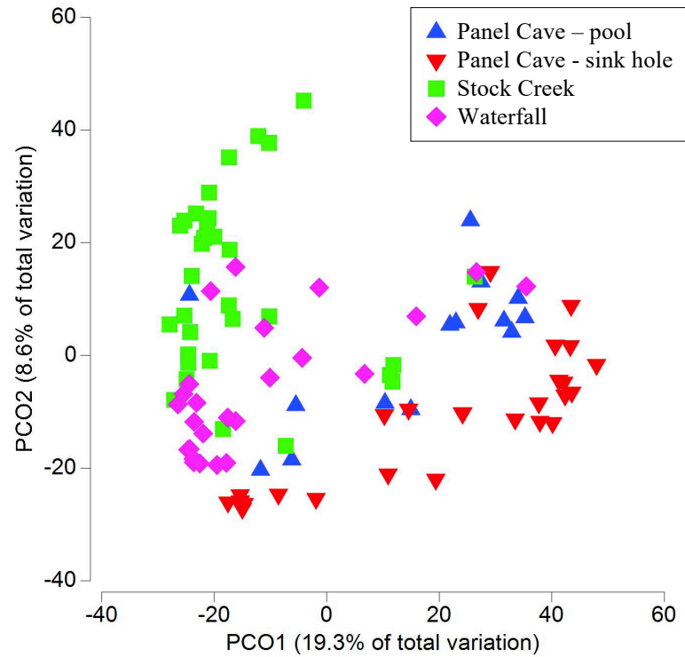
Supplemental Figure 2. PCoA plot of samples collected from Panel Cave and surface sites
