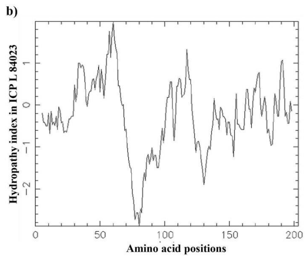
Fig. S1: Kyte and Doolittle hydropathy plot in a) ICP 7035 and b) ICPL 84023
