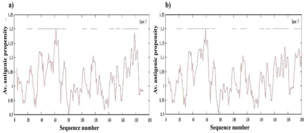
Fig. S3: Average antigenic propensity in a) ICP 7035 and b) ICPL 84023
