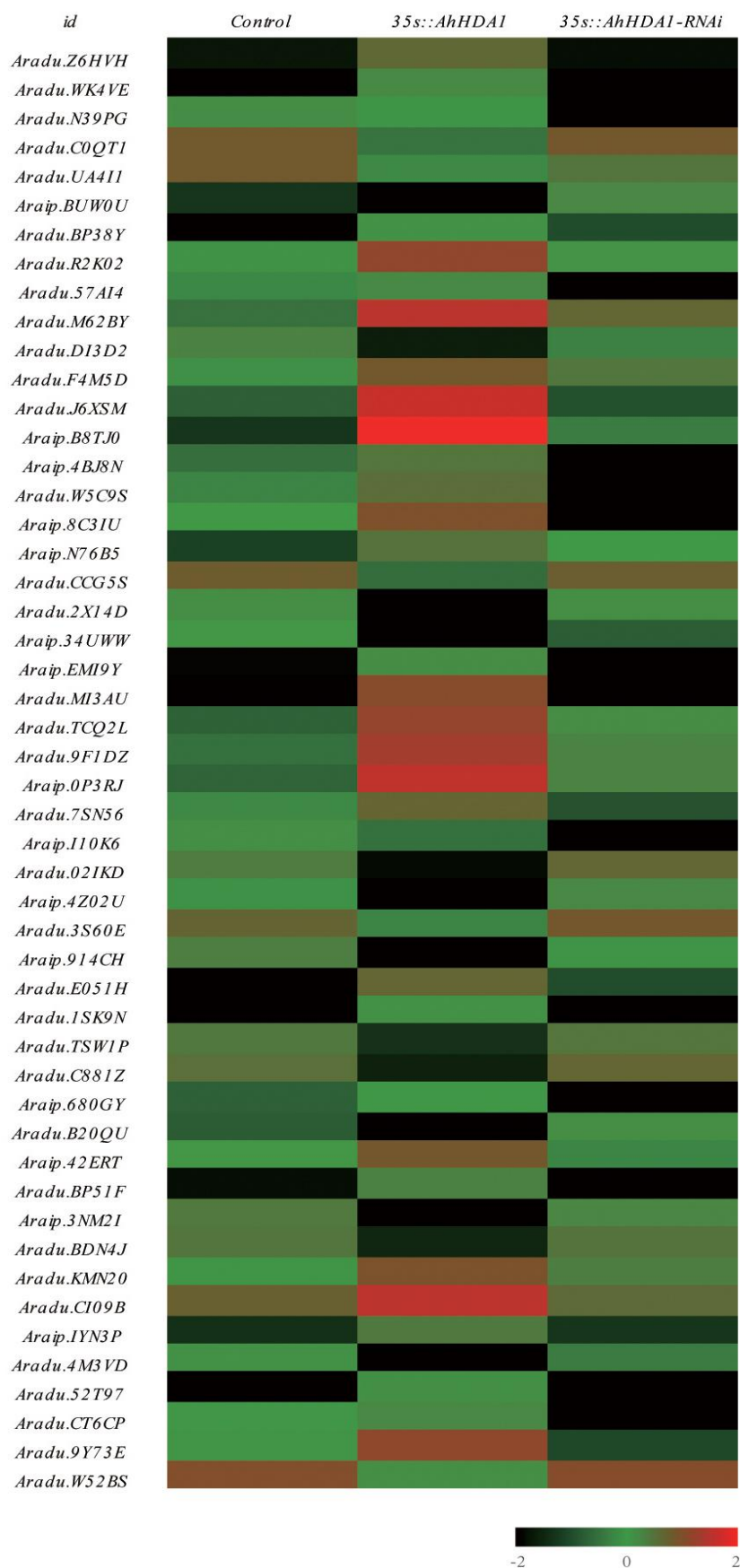
Figure S1 Heatmap of substance synthesis and energy metabolism pathway among different hairy roots.
