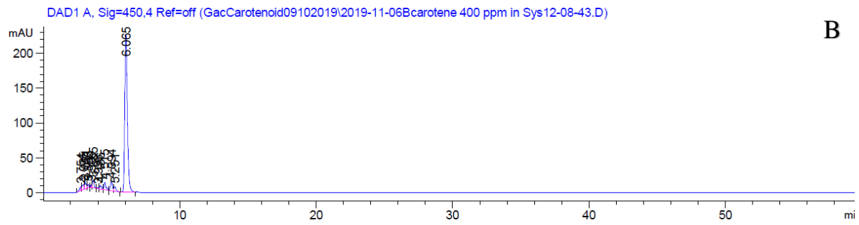
\beta -carotene (A) and lycopene (B) standard at 450 nm.
