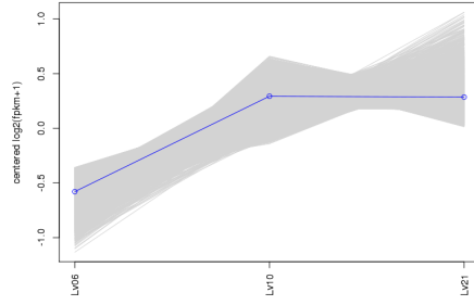
subcluster_8_log2_medianCentered_fpkm.matrix, 6092 trans
