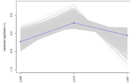
subcluster_5_log2_medianCentered_fpkm.matrix, 10253 trans
