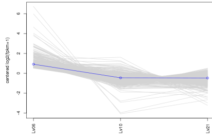
subcluster_5_log2_medianCentered_fpkm.matrix, 10253 trans
