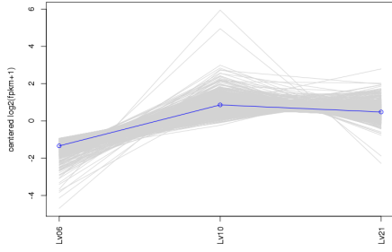
subcluster_7_log2_medianCentered_fpkm.matrix, 1073 trans
