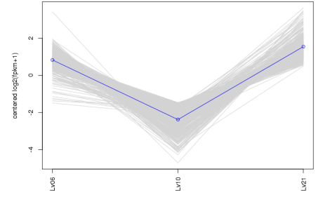
subcluster_9_log2_medianCentered_fpkm.matrix, 498 trans
