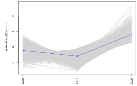
subcluster_6_log2_medianCentered_fpkm.matrix, 6909 trans
