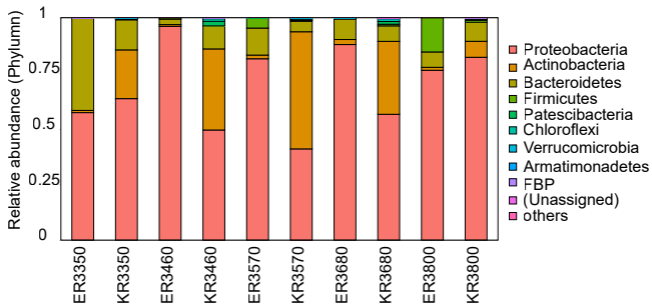
(A) Bacteria
