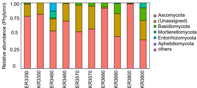
(B) Fungi
