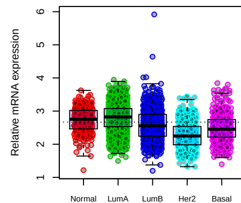
METTL16
