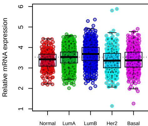
METTL3
