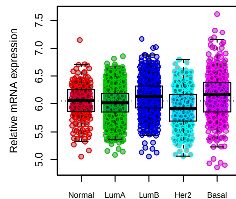
RBMX
