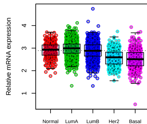
METTL14
