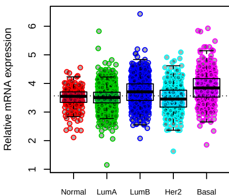
FMR1
