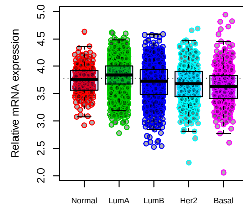
RBM15B
