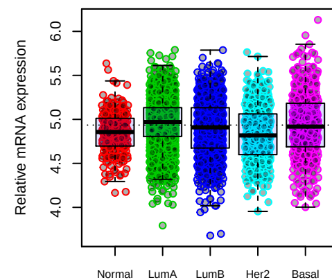
YTHDF2
