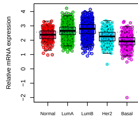
YTHDC2
