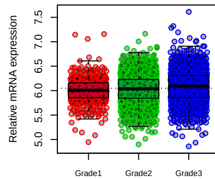
RBMX
