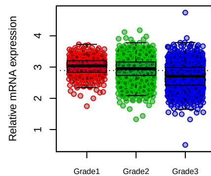
METTL14
