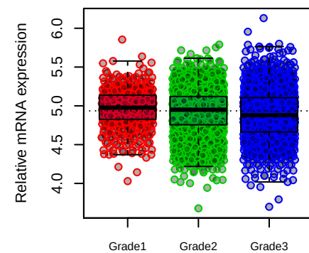
YTHDF2
