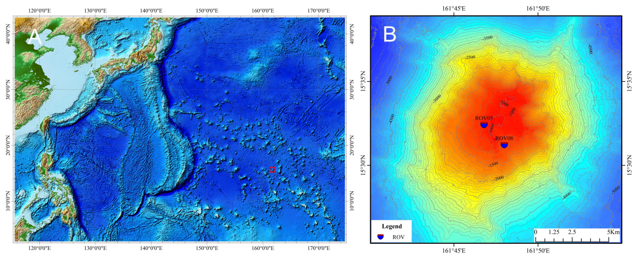
Figure 1 Map of the RC seamount (indicated by the small red block) in the northwest Pacific (A) and sampling sites of specimens of ophioplithacids (B).
