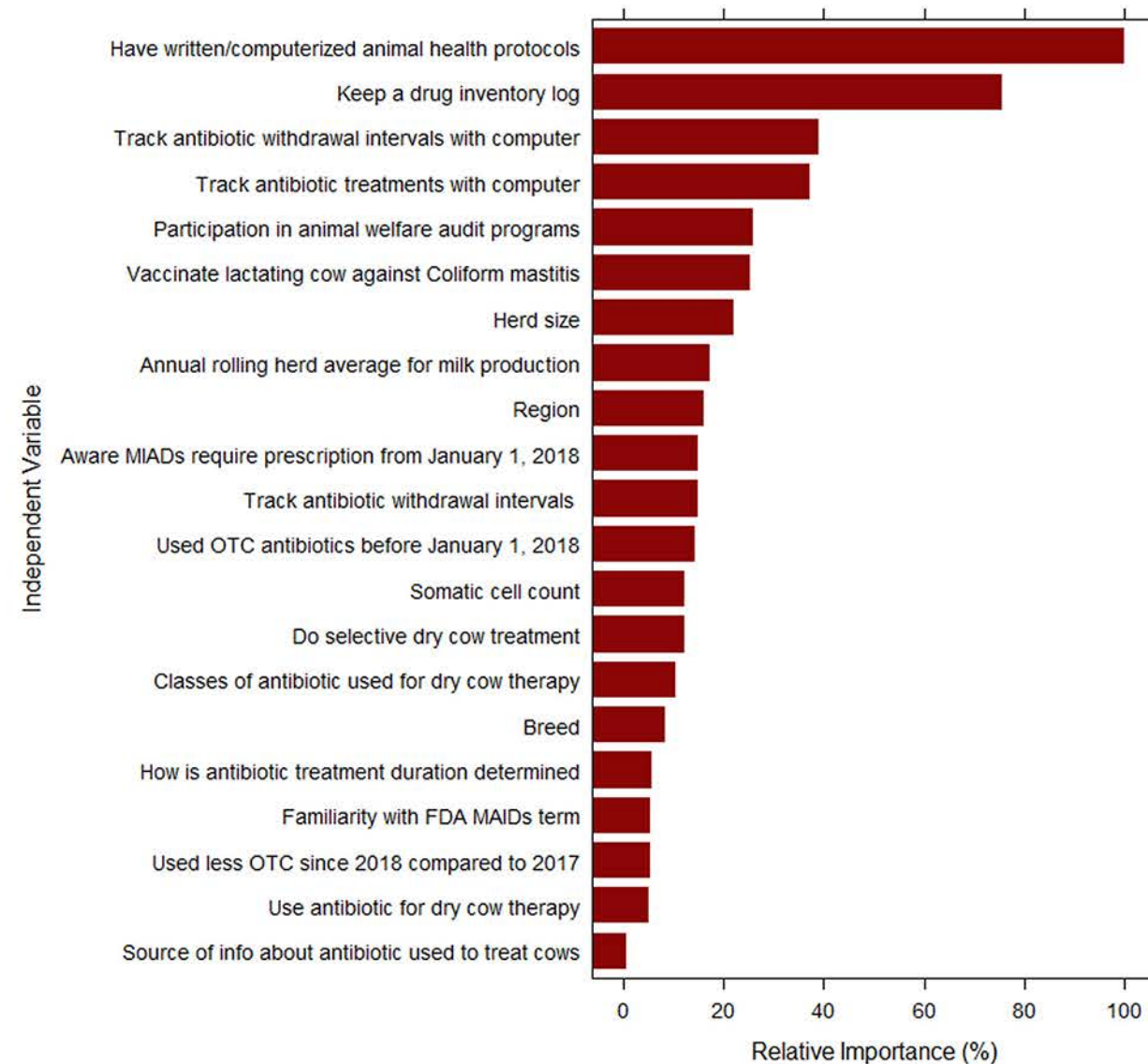
Decision Tree Model
