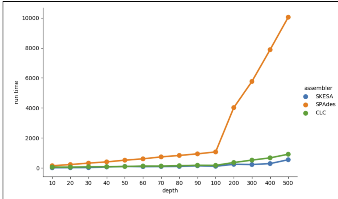
Figure S1. The estimation of the minimum read coverage for the running time of SPAdes, CLC, and SKESA assemblers. Comparison of different read lengths for the assembling running time according to different simulated read coverages among SPAdes, CLC, and SKESA for S. enterica LT2.
