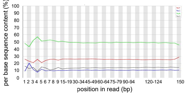
Ring method1 enriched HiSeq
