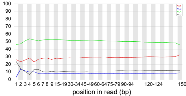
Trophozoite method1 unenriched HiSeq
