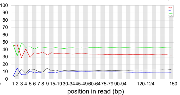
Schizont method2 unenriched HiSeq
