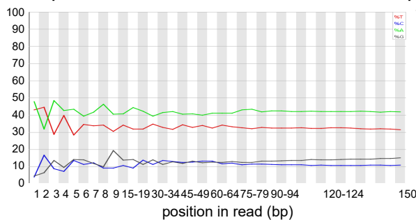
Trophozoite method2 unenriched HiSeq
