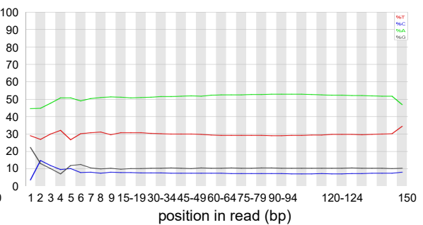
Schizont method1 enriched HiSeq
