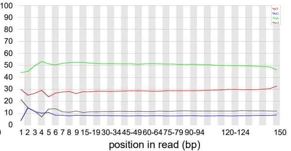
Schizont method1 unenriched HiSeq
