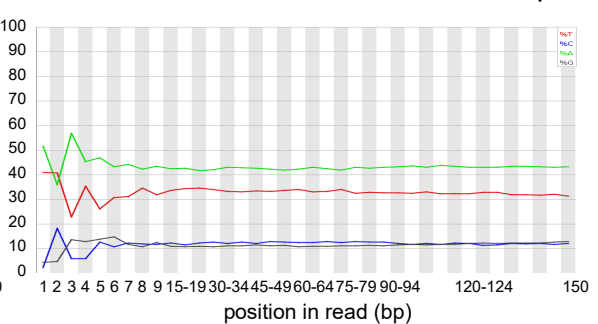
Schizont method2 enriched HiSeq
