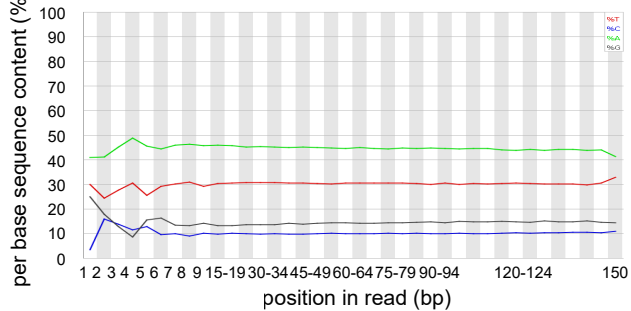
Ring method1 unenriched HiSeq
