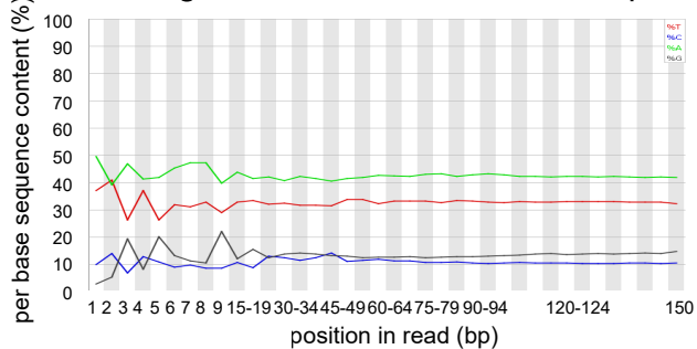
Ring method2 unenriched HiSeq
