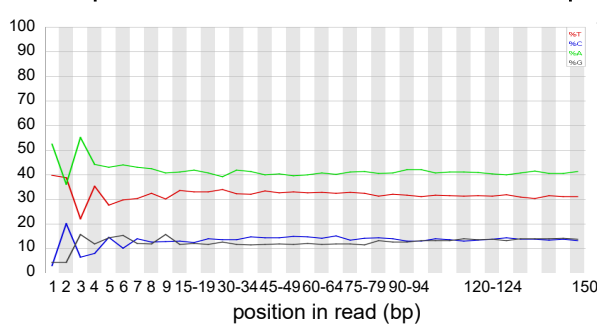
Trophozoite method2 enriched HiSeq
