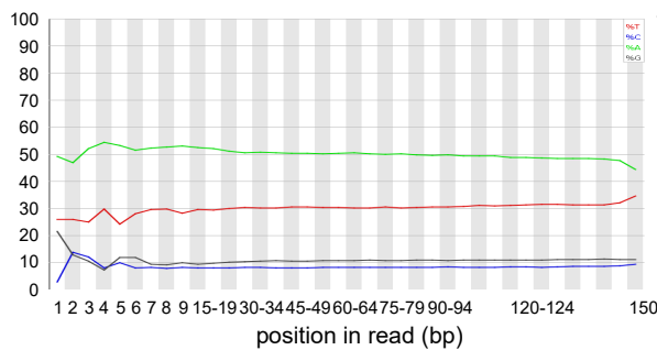
Trophozoite method1 enriched HiSeq
