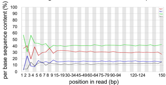
Ring method2 enriched HiSeq
