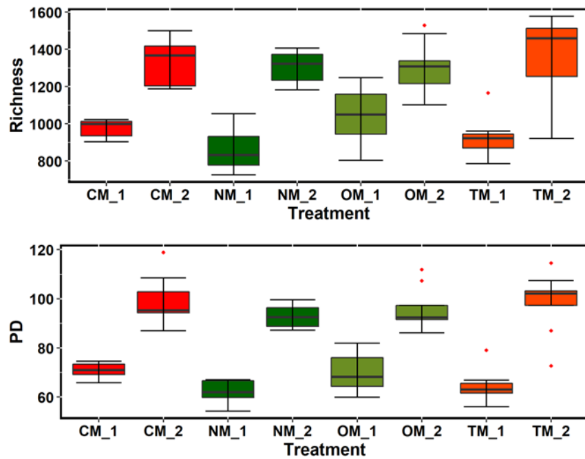
Supplementary Figure 2 Boxplot of the diversity indices. The lower and upper box boundaries represent the 25th and 75th percentiles, respectively, the central line stands for the inside box median. CM: conventional management, TM: transition management, OM: organic management, NM: natural management. _1: Year 1, _2: Year 2. PD is the Faith's phylogenetic diversity and Richness is the observed ASVs numbers. Red dots representing outliers.
