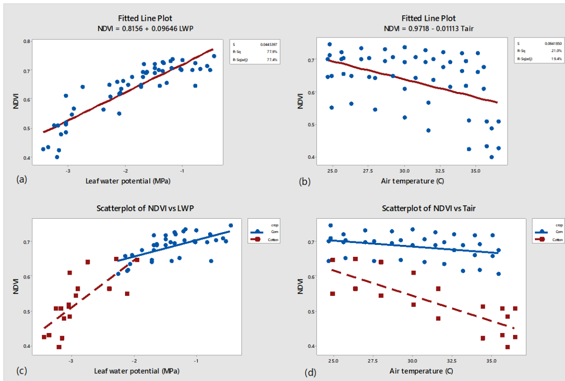
Figure S5. A comparison of the relationship between NDVI and leaf water potential (LWP) and that of the NDVI and air temperature (°C) for combined data of corn and cotton measured in 2018.
