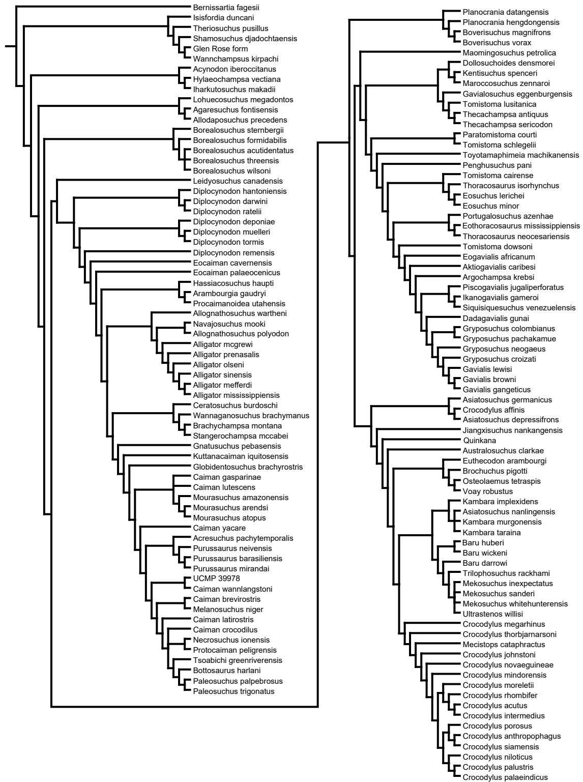
Figure 8: Strict consensus of 3 MPTs from Analysis 3.3
