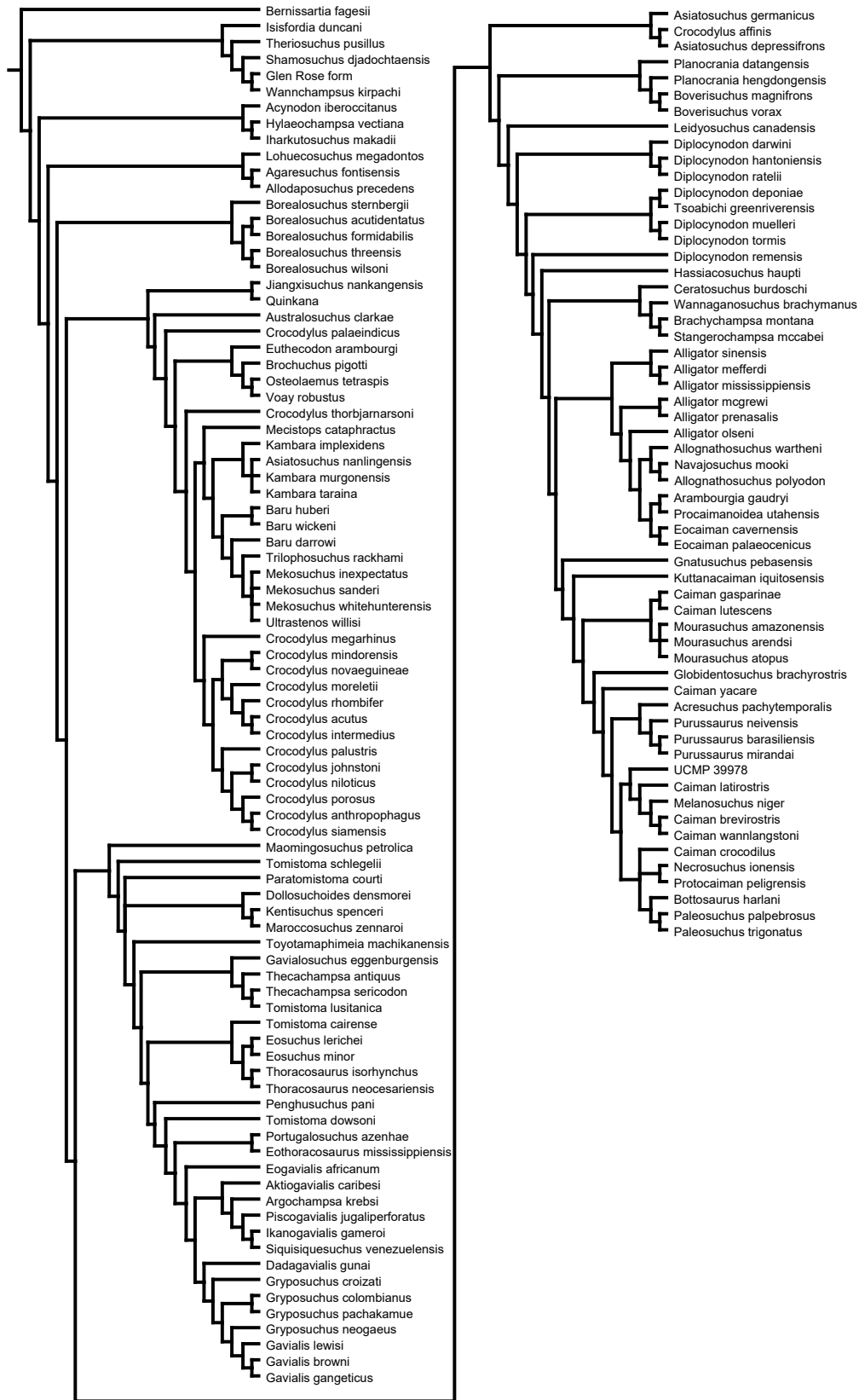
Figure 4: Strict consensus of 3 MPTs from Analysis 2.2
