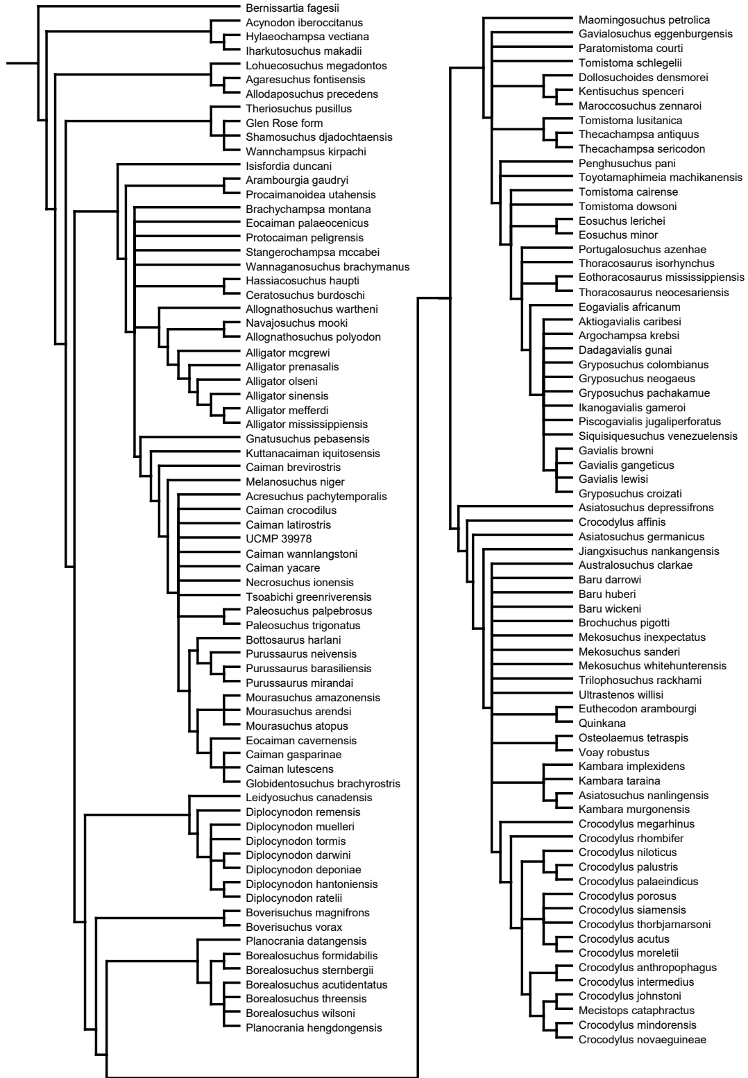
Figure 3: Strict consensus of 400,000 MPTs from Analysis 2.1
