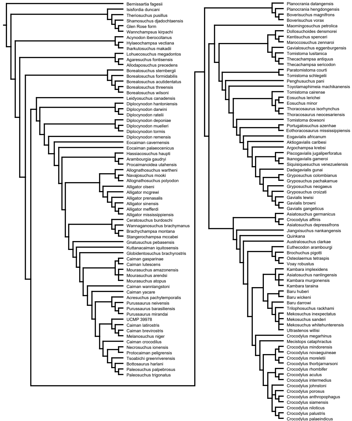
Figure 5: Strict consensus of 3 MPTs from Analysis 2.3
