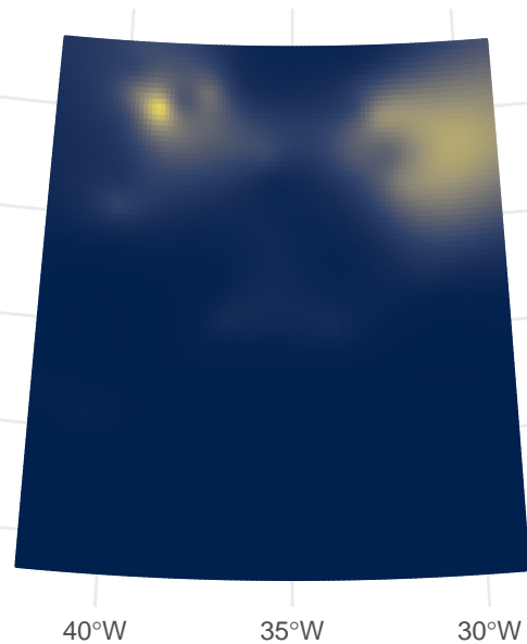
Factor swim
