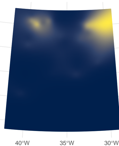
Factor-smooth swim
