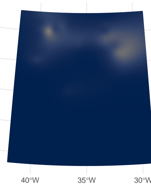
Factor-smooth fly
