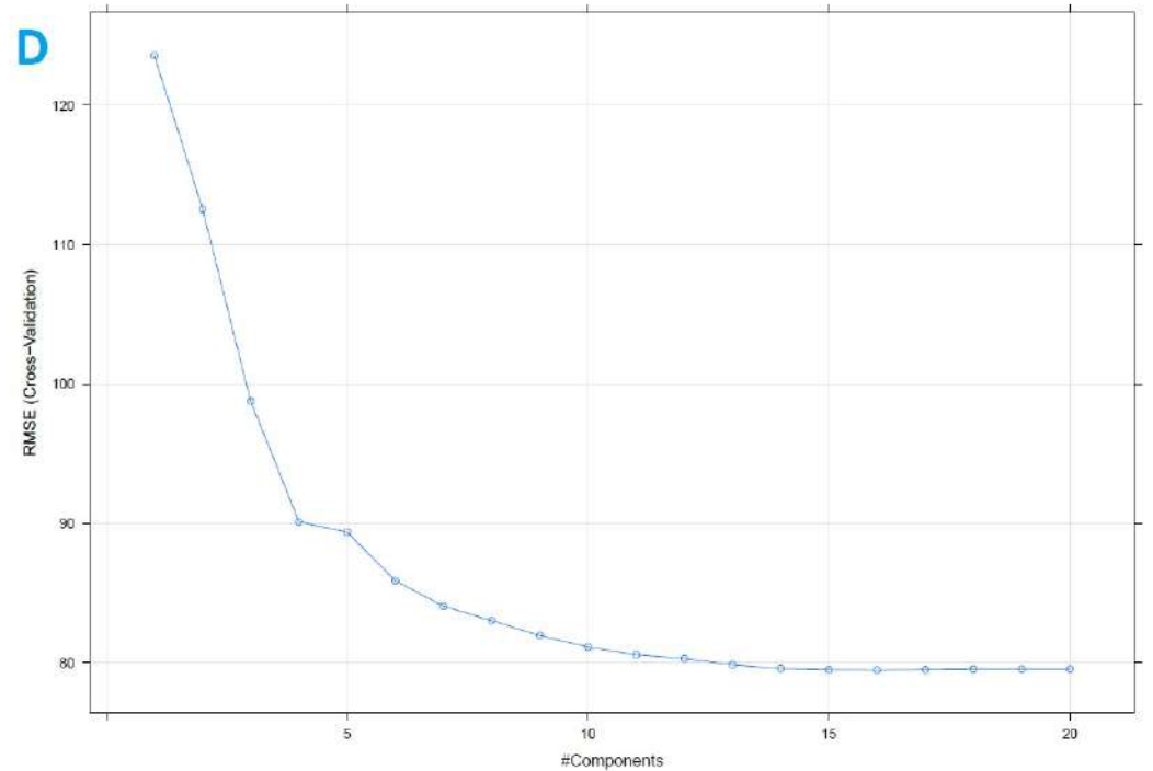
Maltose: PCR - Standardized data (a), PCR - Augmented data (b), PLS - Standardized data (c), and PLS - Augmented data (d)
