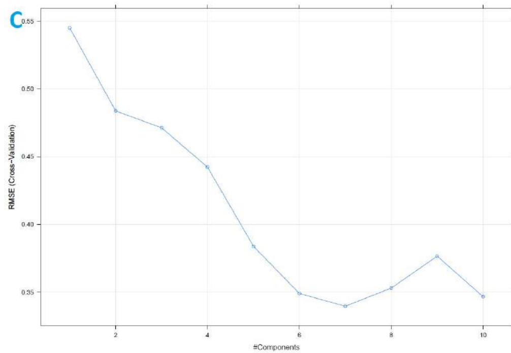
Sucrose: PCR - Standardized data (a), PCR - Augmented data (b), PLS - Standardized data (c), PLS - Augmented data (d)
