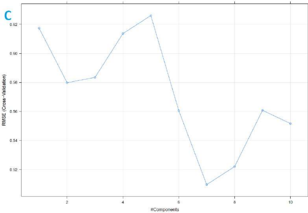
Fructose: PCR - Standardized data (a), PCR - Augmented data (b), PLS - Standardized data (c), and PLS - Augmented data (d)
