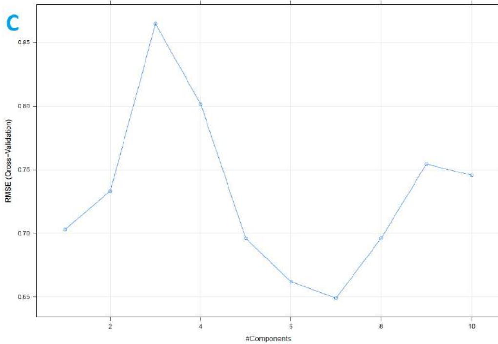
Maltose: PCR - Standardized data (a), PCR - Augmented data (b), PLS - Standardized data (c), and PLS - Augmented data (d)
