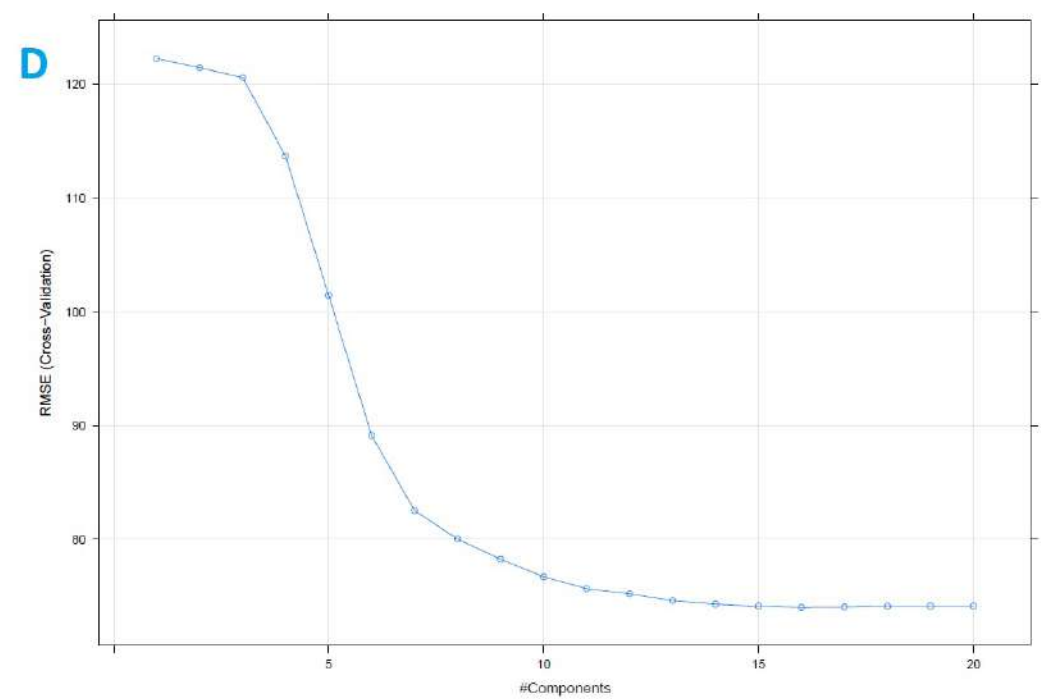
Sucrose: PCR - Standardized data (a), PCR - Augmented data (b), PLS - Standardized data (c), PLS - Augmented data (d)
