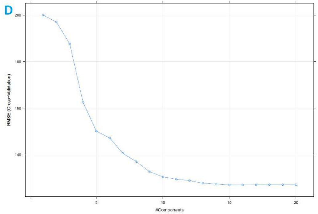
Fructose: PCR - Standardized data (a), PCR - Augmented data (b), PLS - Standardized data (c), and PLS - Augmented data (d)
