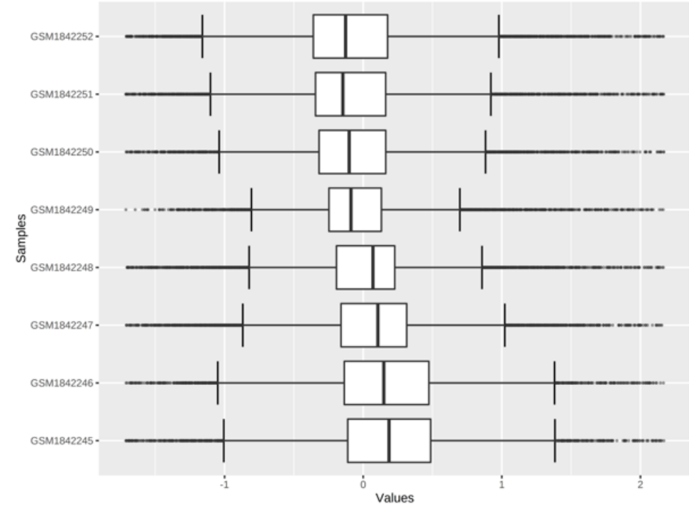
GSE71647
