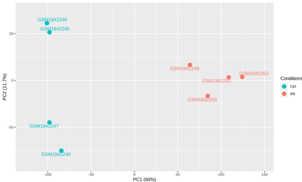
GSE71647
