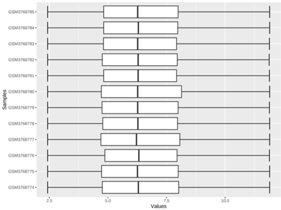
GSE131288
