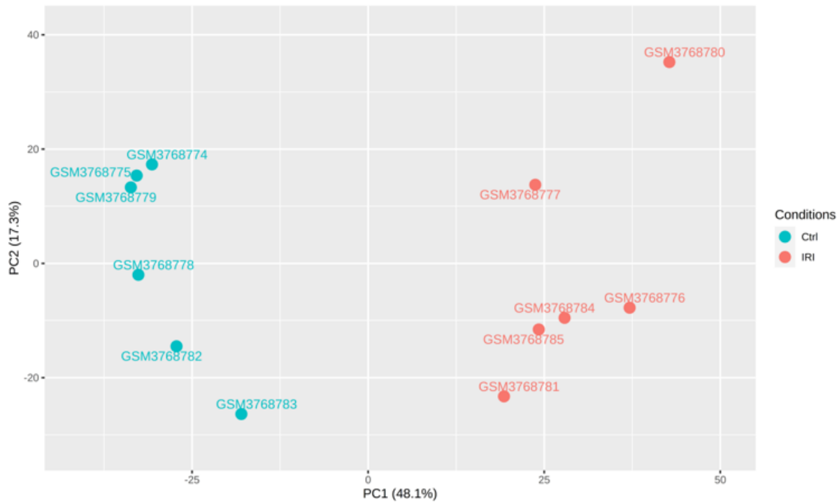
GSE131288
