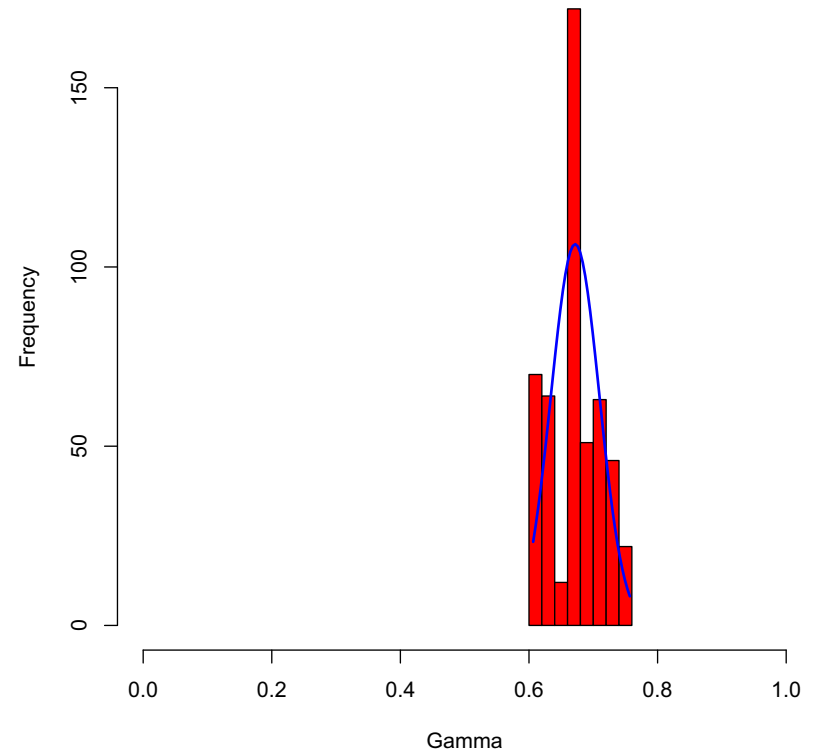
B HyDe Test, C. douglasii as AMER × SANG hybrid 500 bootstrap replicates
