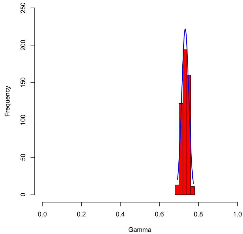
A HyDe Test, C. rivularis as AMER × SANG hybrid 500 bootstrap replicates
