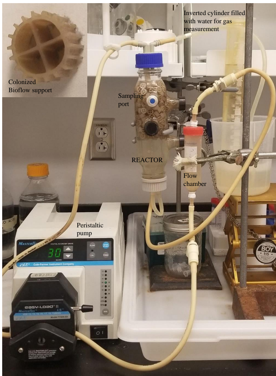
Figure S1. Configuration of the reactor
