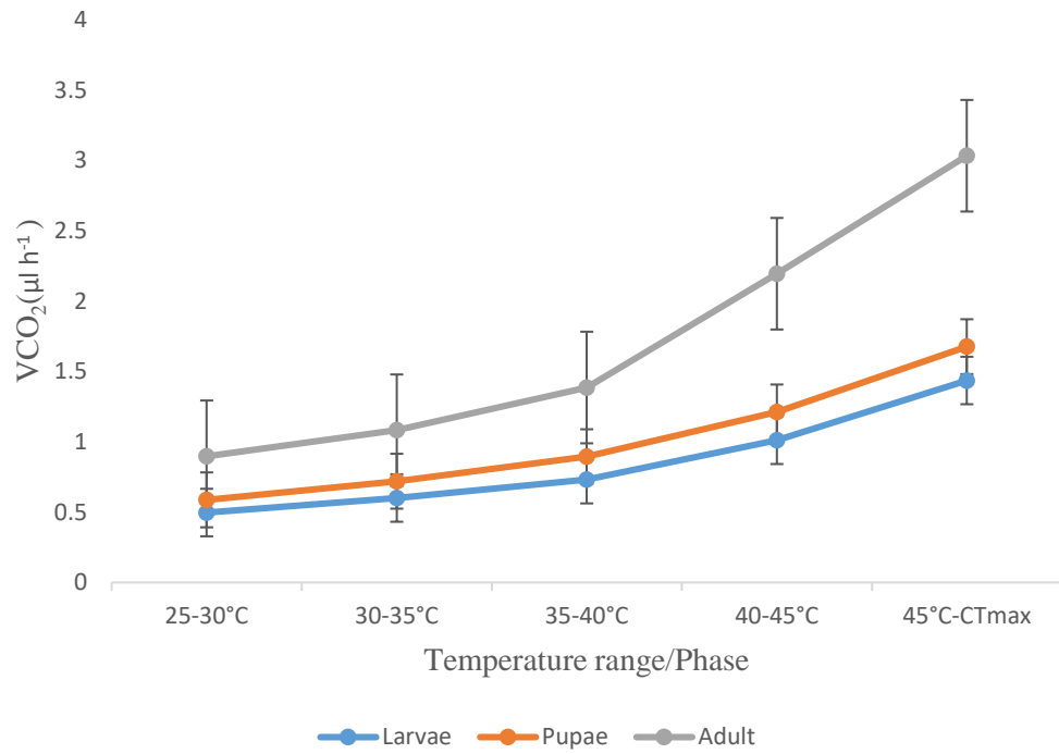
Figure 2. Effect of different temperature phases on VCO 2 in H. punctigera life stages (Larvae, Pupae and Adult) during thermolimit respirometry. Points are means ± s.e.m.
