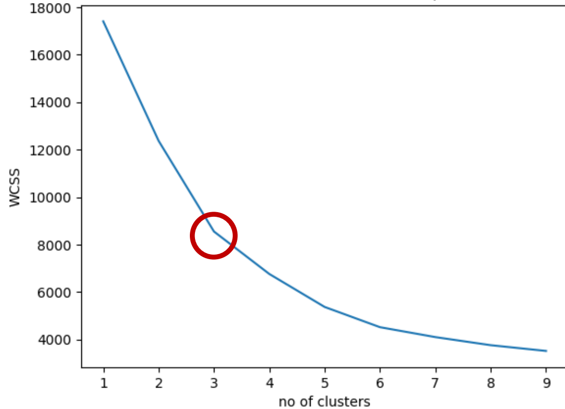
Elbow Method for Sick Group
