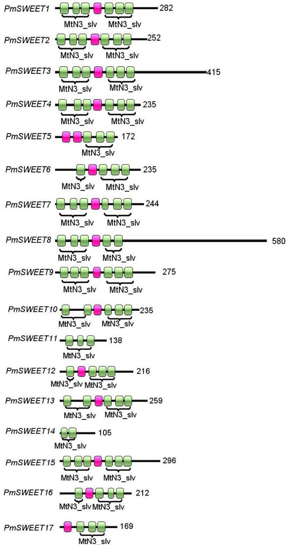
Supplementary Figure 1. Schematic representation of PmSWEET proteins. Colored boxes indicate TMs. The IBS1.0 software was used to drawing diagram (Liu et al., 2015).
