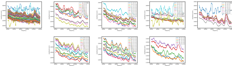
Figure 9: LSTM200. Fouriers on reference-base probability for chromosome: hg38_chr20. The genome string is divided in adjacent segments of 1Mb; several adjacent segments are covered in each plot, segment numbers are indicated in the legend. First plot (upper left) shows the results for all segments in this chromosome.
