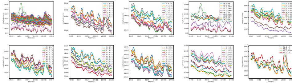
Figure 6: LSTM200. Fouriers on reference-base probability for chromosome: hg38_chr17. The genome string is divided in adjacent segments of 1Mb; several adjacent segments are covered in each plot, segment numbers are indicated in the legend. First plot (upper left) shows the results for all segments in this chromosome.
