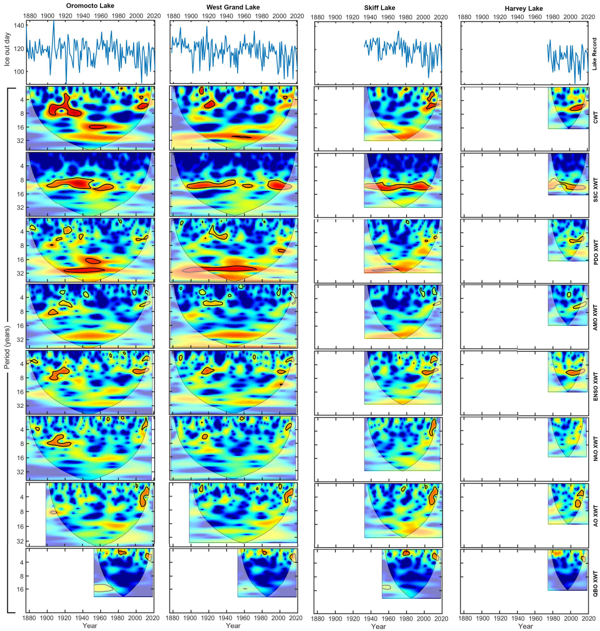
Figure S1: Graphical representation and the continuous wavelet transform (CWT) for Oromocto Lake. Cross wavelet transforms (XWTs) between lake ice out records and each of the SSC, PDO, AMO, ENSO, NAO, AO, and QBO. Time scales all span 1876–2020 for easy comparisons between the CWTs and XWTs.
