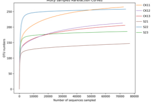
Multi samples Rarefaction Curves
