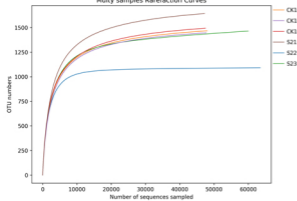
Multi samples Rarefaction Curves
