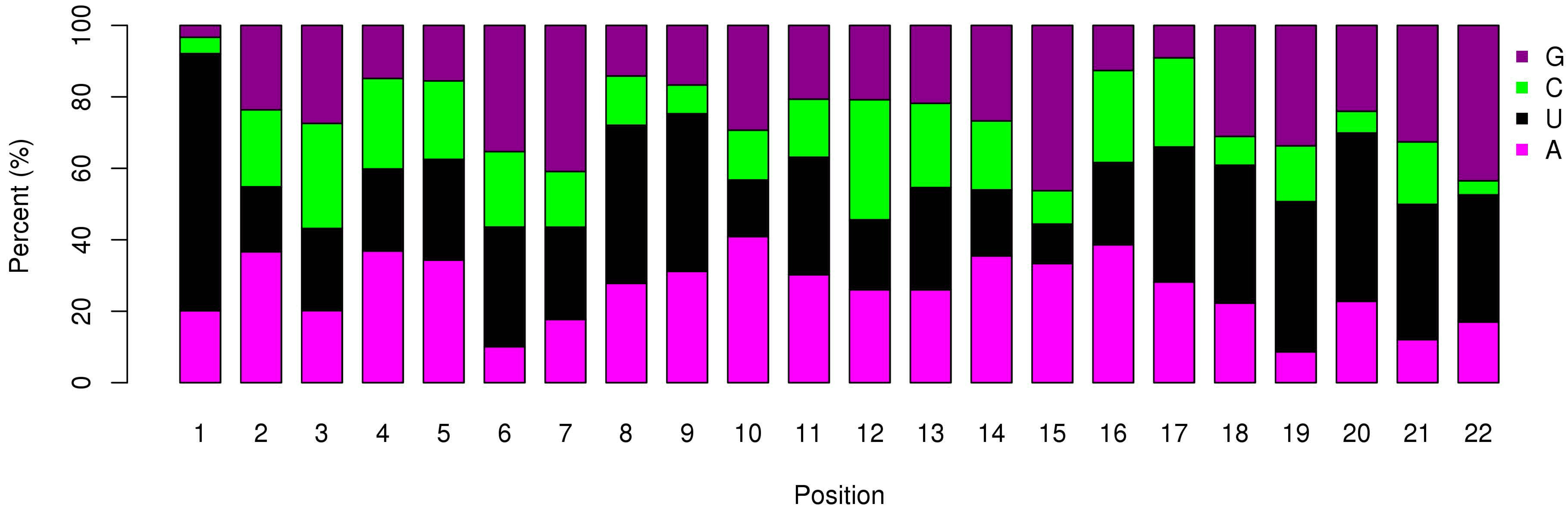
miRNA Nucleotide Bias at Each Position (S_D_A)
