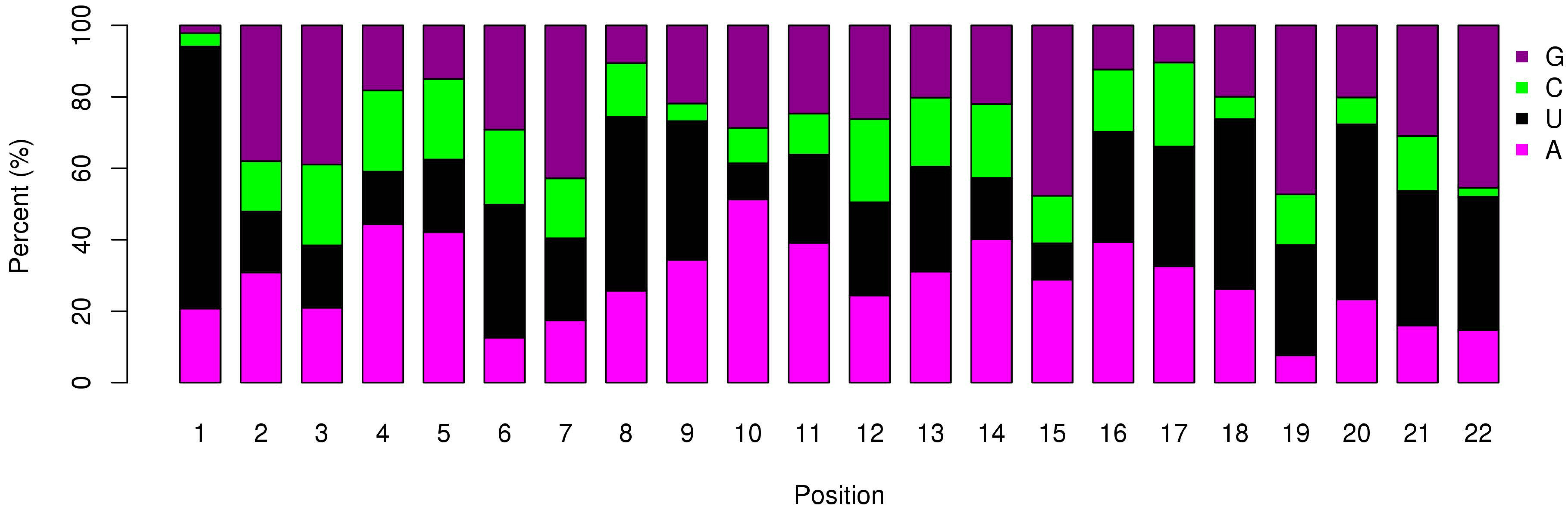
miRNA Nucleotide Bias at Each Position (T_D_A)
