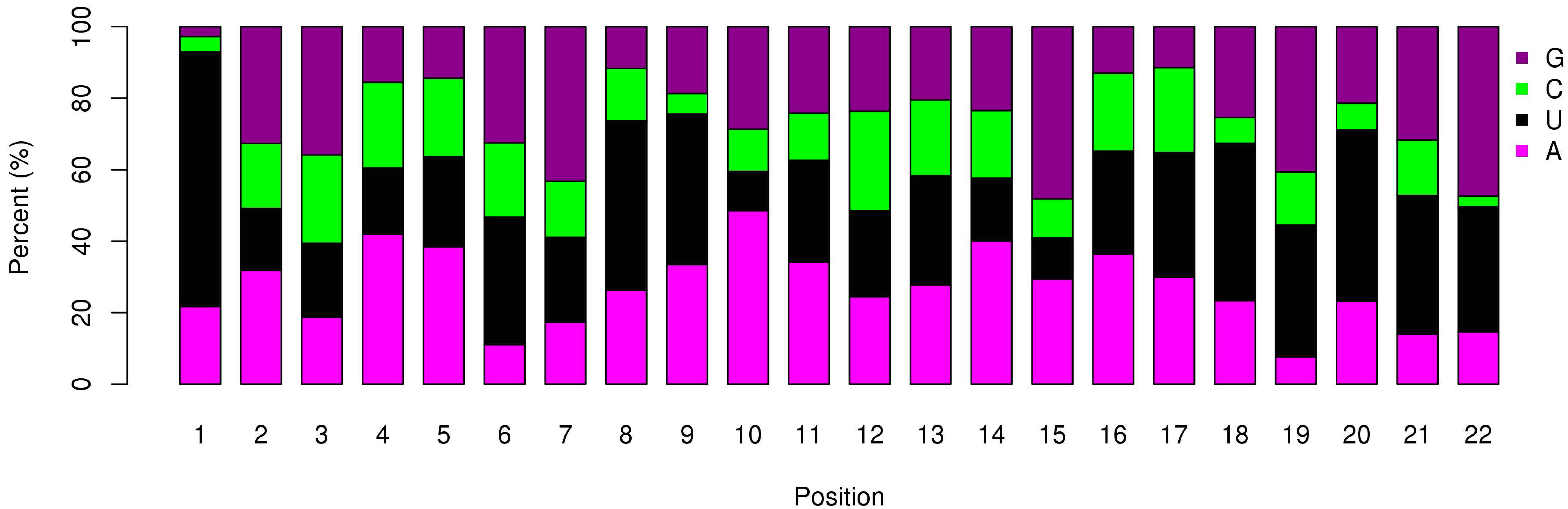
miRNA Nucleotide Bias at Each Position (T_D_B)
