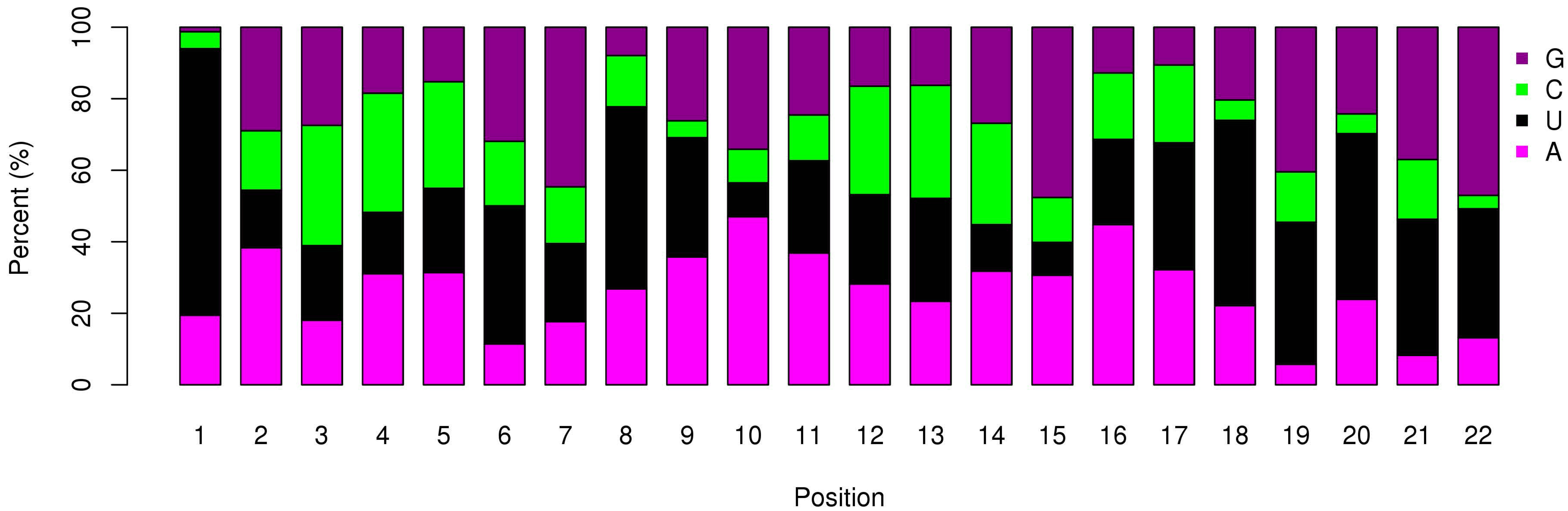
miRNA Nucleotide Bias at Each Position (S_D_B)
