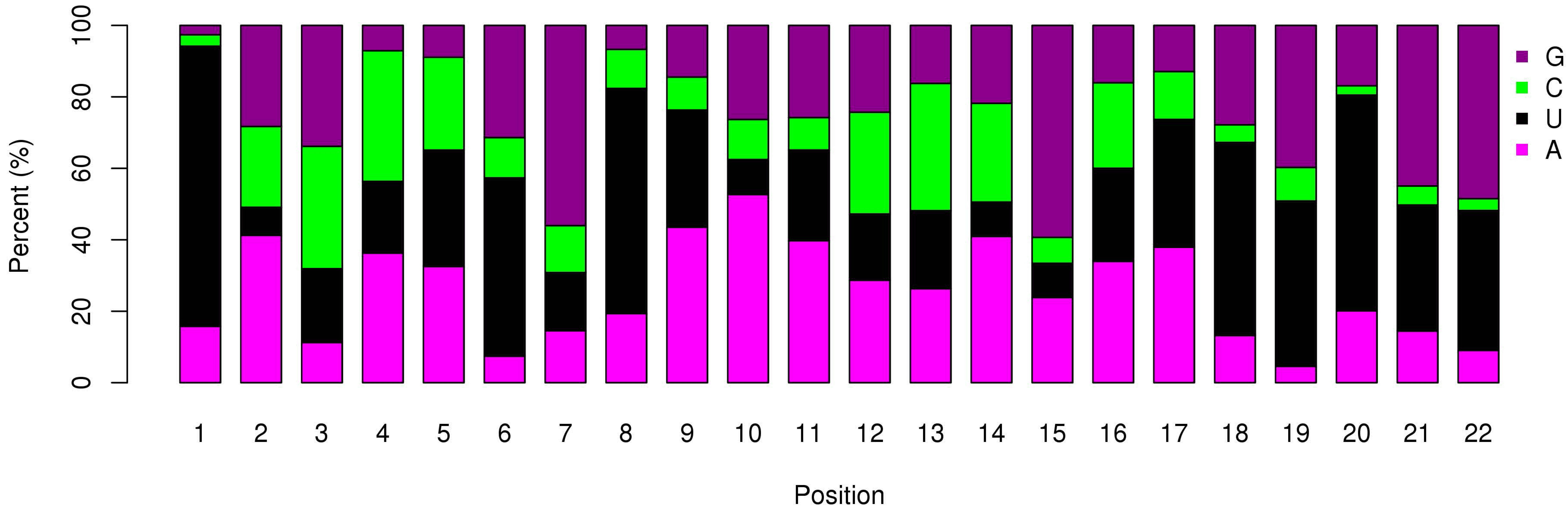
miRNA Nucleotide Bias at Each Position (O_D_B)
