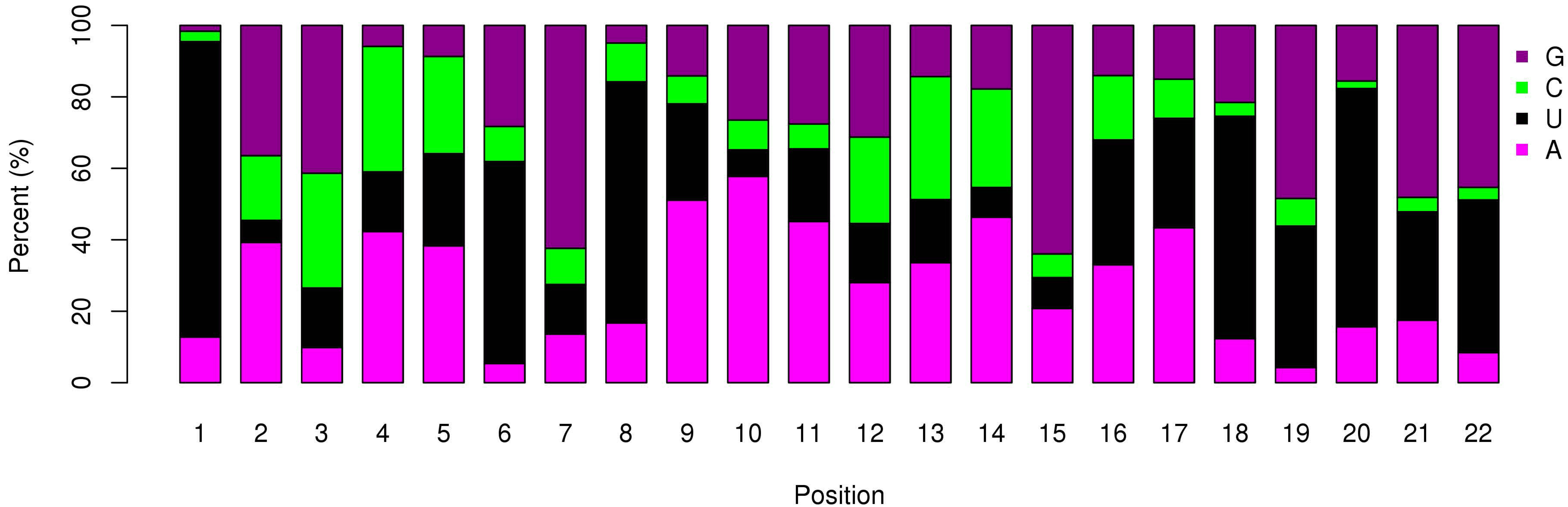
miRNA Nucleotide Bias at Each Position (O_D_A)
