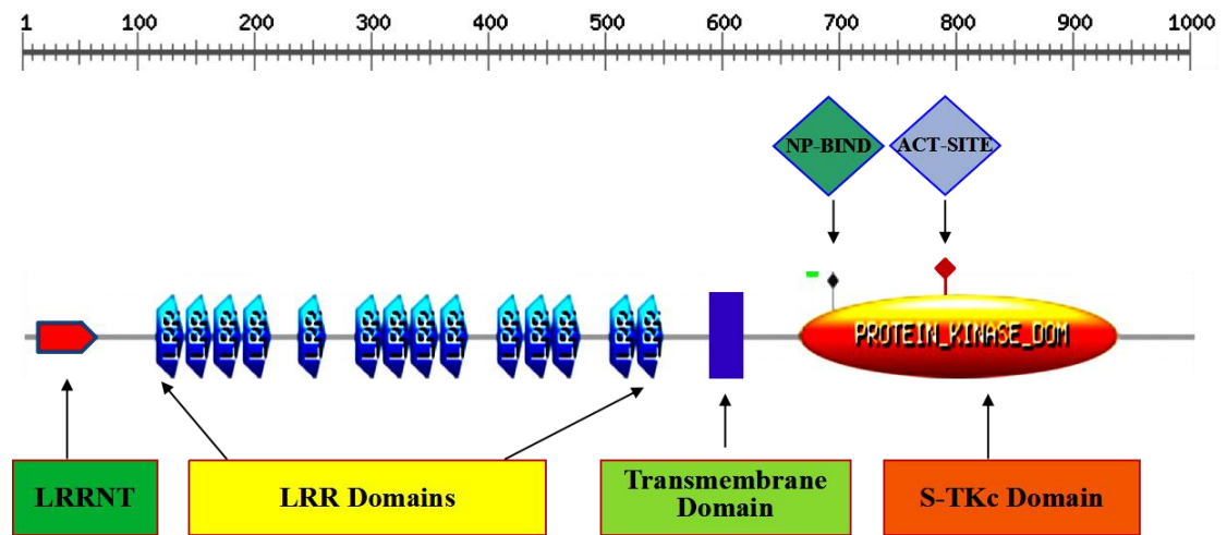
Annex 5 Figure S2 The conserved structure domain of SiER family members
