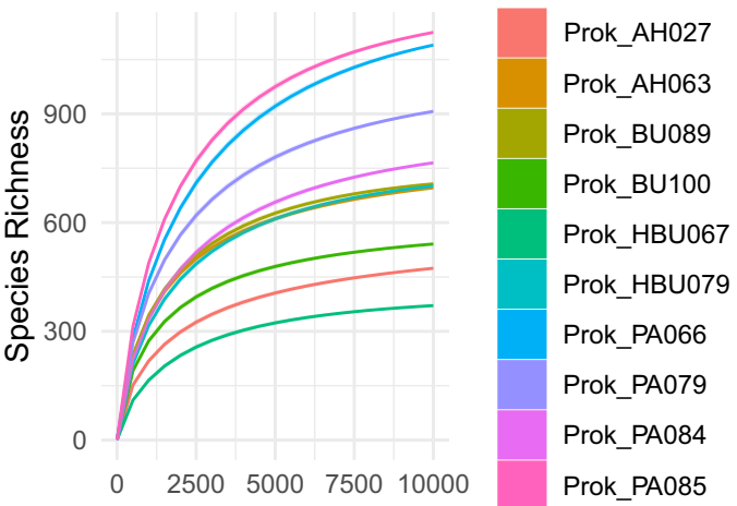
Prok 10,000 sequences
