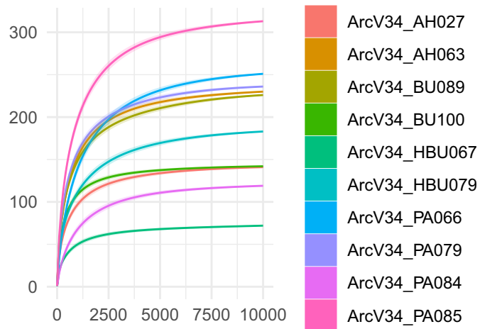
V34 10,000 sequences
