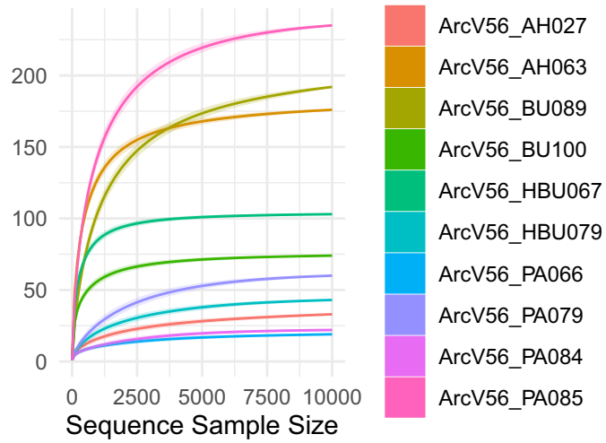
V56 10,000 sequences
