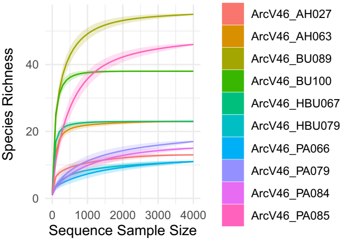
V46 4,000 sequences
