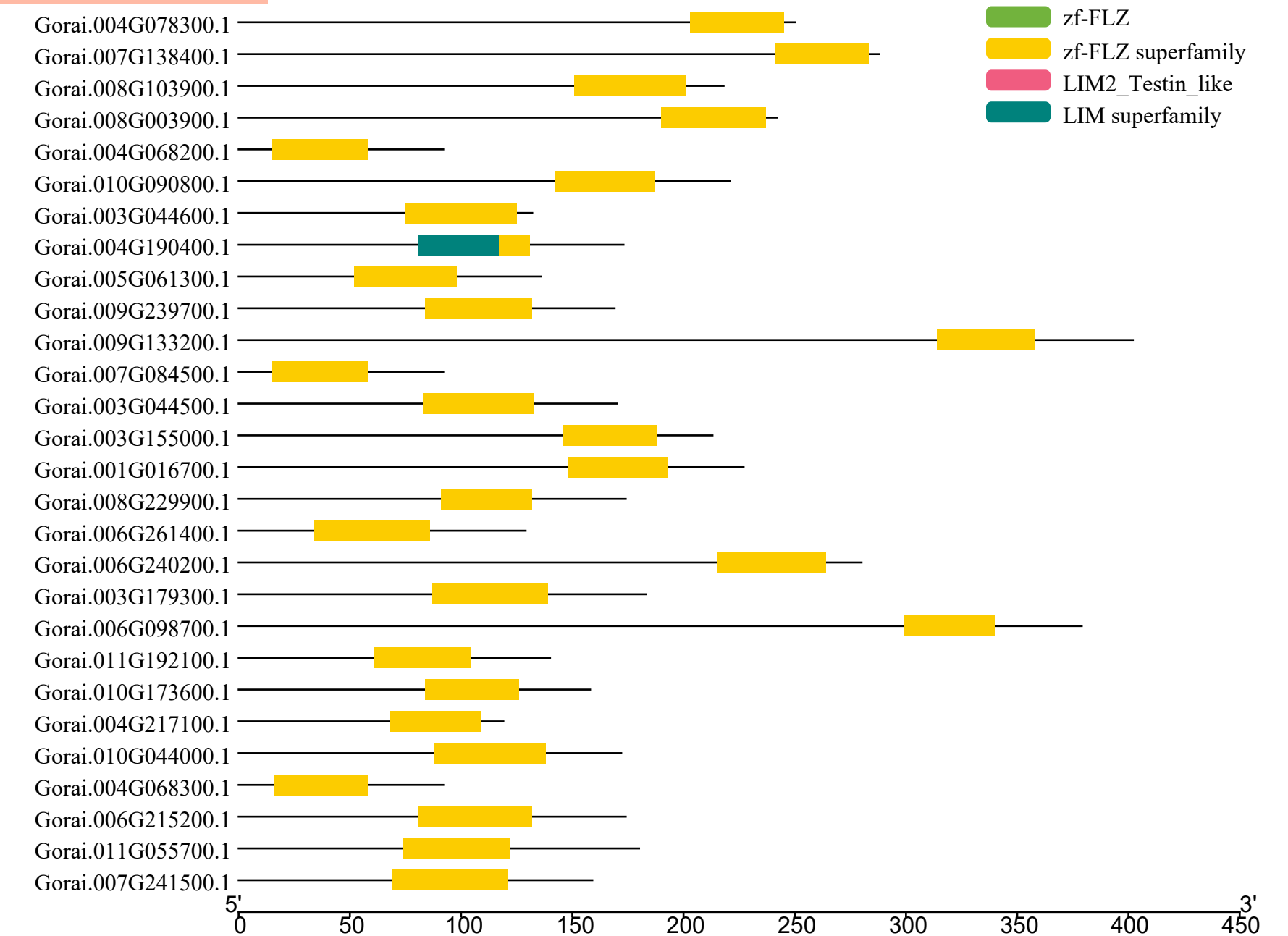
Fig S1. Distribution of the FLZ domain in the FLZ proteins of cotton.
