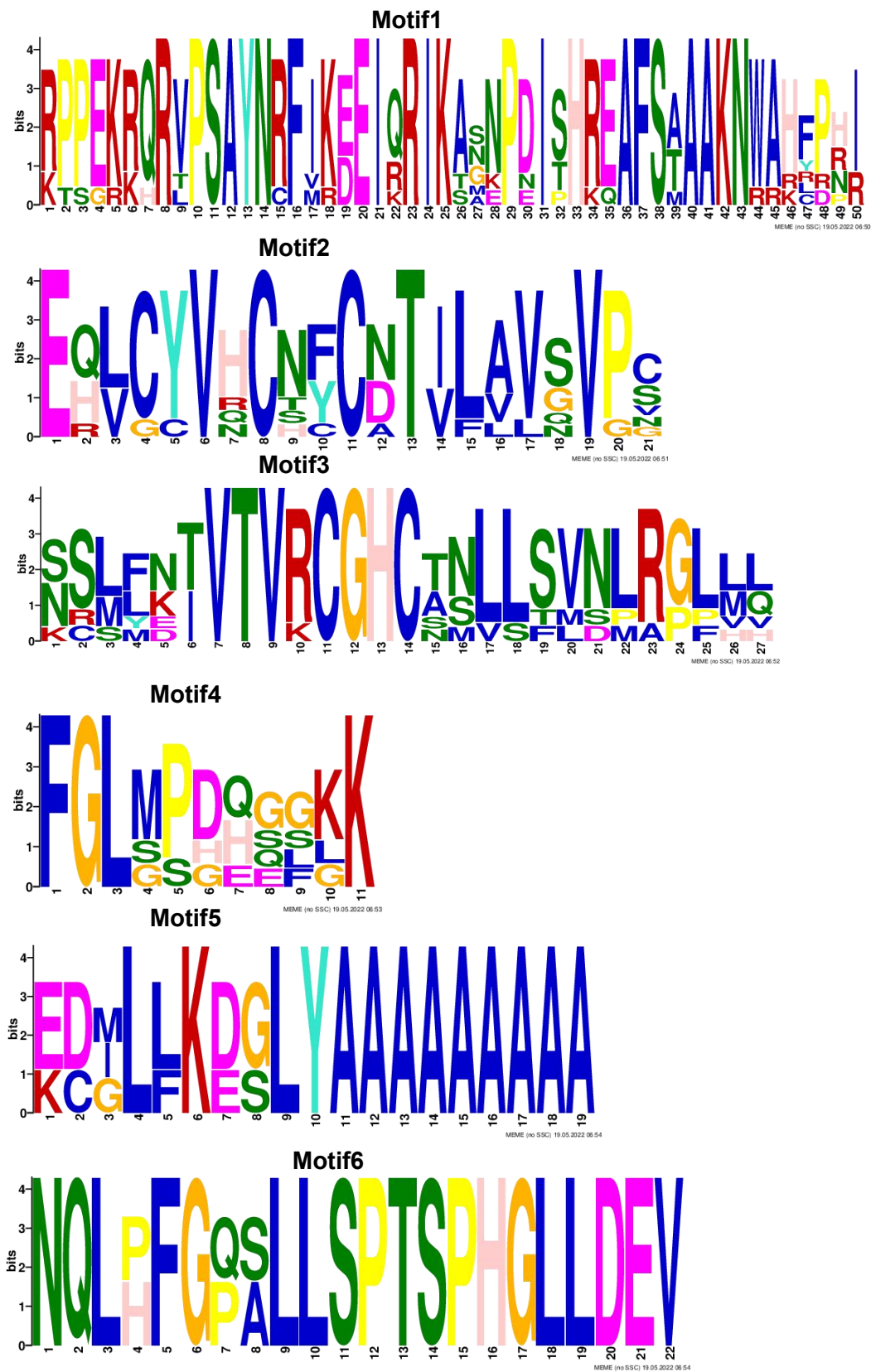
Figure S2 Motif sequences of OsYABBYs detecting by MEME.
