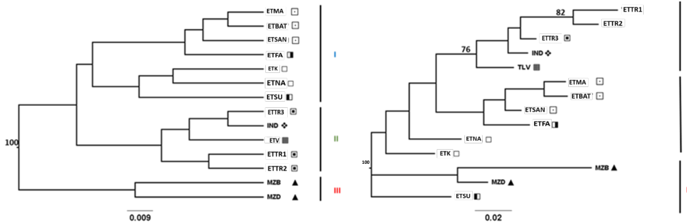
Supplementary Figure S1. UPGMA (A) and NJ (B) trees generated using matrix Nei's D distance, respectively, representing the cashew populations from East Timor, Indonesia, and Mozambique.
