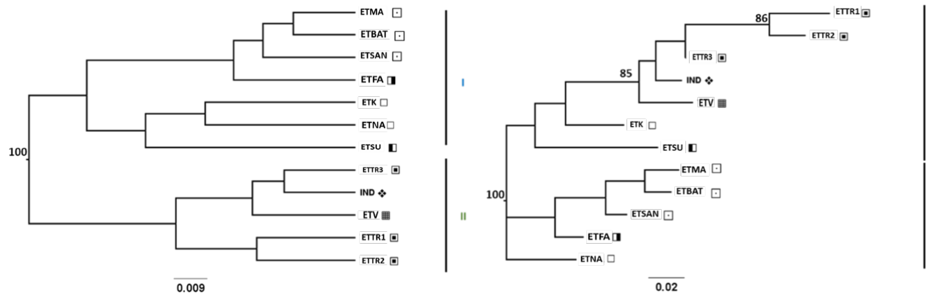
Supplementary Figure S2. UPGMA (A) and NJ (B) trees generated using matrix Nei's D distance, respectively, representing the cashew populations of East Timor and Indonesia .
