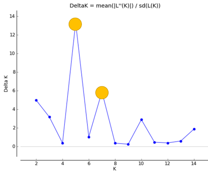
Supplementary Figure S3. STRUCTURE ad hoc statistics retrieved by Structure_Harvester using 1 to 15 possible clusters ( K ). Variation of \Delta K values according to the method outlined by Evanno et al. (2005) for populations from East Timor, Indonesia and Mozambique.
