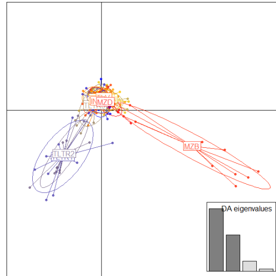
Supplementary Figure S5. Scatterplot of the DAPC analysis of K = 5 assignment . Scatterplot shows the two principal components of the DAPC, and clusters are numbered and displayed by different colors, while dots represent individuals. The 2 Discriminant Functions hereby represented explain 93% of cumulative variance of the dataset
