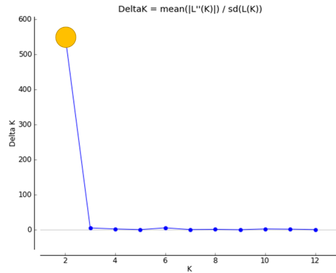
Supplementary Figure S7. STRUCTURE ad hoc statistics retrieved by Structure_Harvester using 1 to 12 possible clusters ( K ). Variation of \Delta K values according to the method outlined by Evanno et al. (2005) for populations from East Timor and Indonesia.
