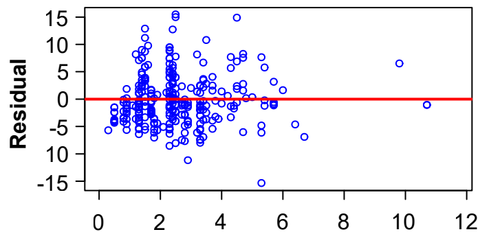
Logistic residuals
