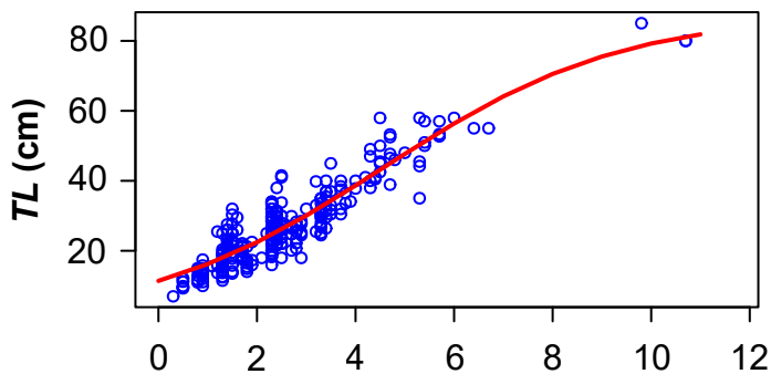
Logistic fit
