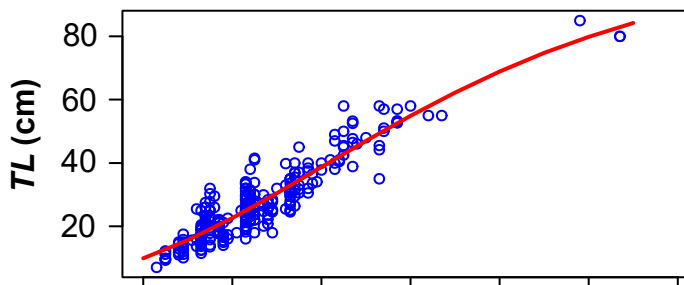
Gompertz fit
