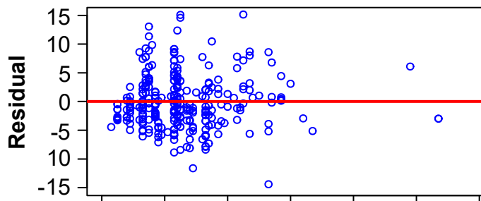
Gompertz residuals
