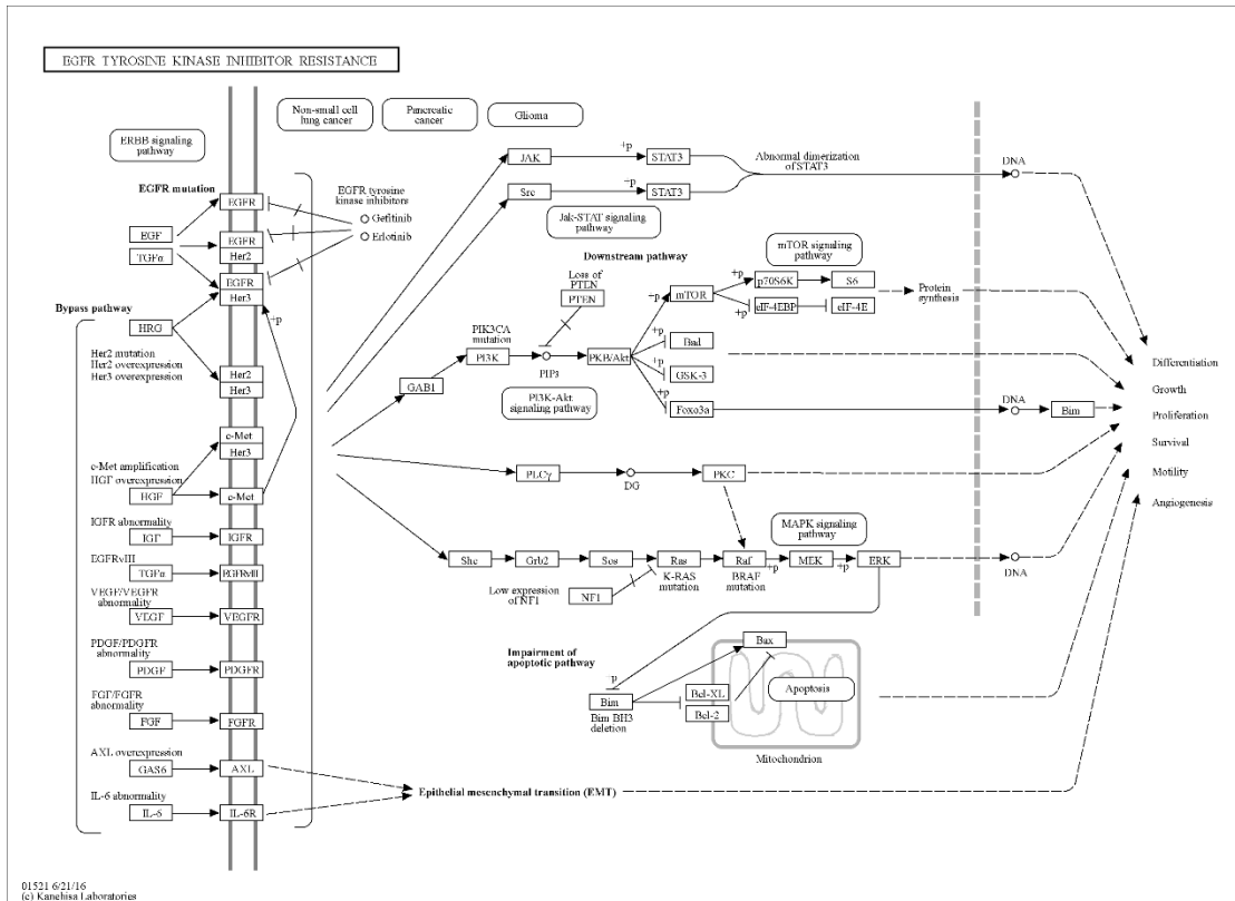
Figure S2. KEGG analysis regulated by Dihyrotanshinone I.
