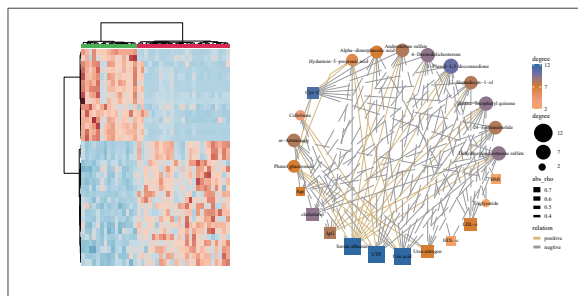
Bioinformatics Analysis
