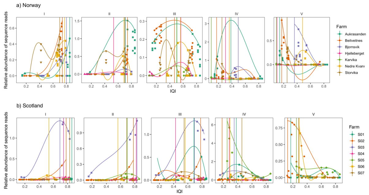
Figure S3 Quantile Regression Spline plots showing the relative abundance of sequences reads of selected bacterial ASVs from Eco-Groups I to V as a function to the Infaunal Quality Index (IQI) for a) Norway salmon farms and b) Scotland salmon farms. Quantile regression splines were constructed at the 95th percentile ( df = 3 ). The IQI value at which the ASV has its peak abundance within a farm is indicated with a vertical line.
