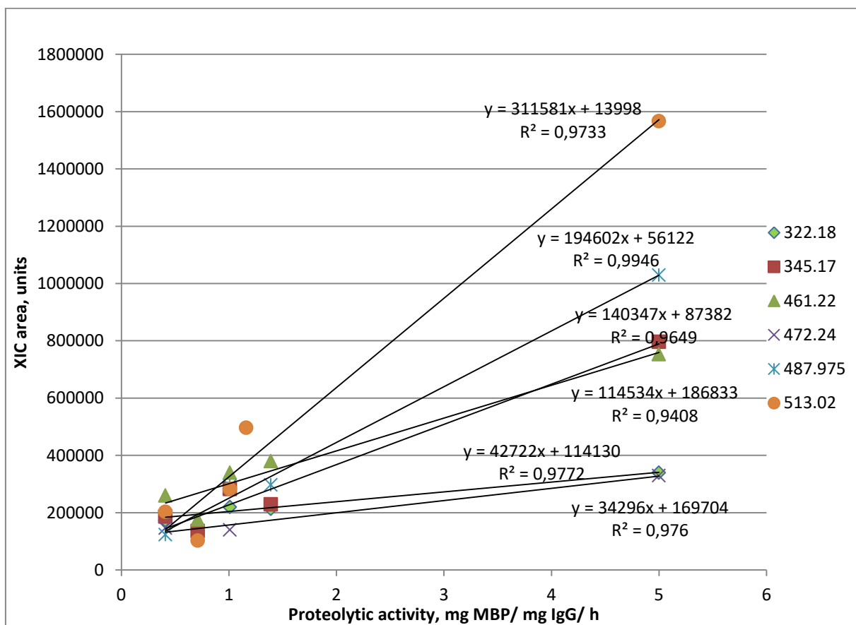
Figure S1. Dependence of the abundance of selected features on proteolytic activity of IgG against MBP.
