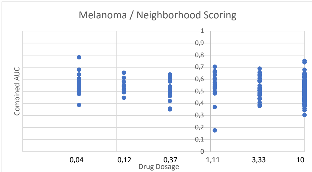
i) Distribution of AUC values with corresponding drug dosages in melanoma (using Neighborhood Scoring-2)
