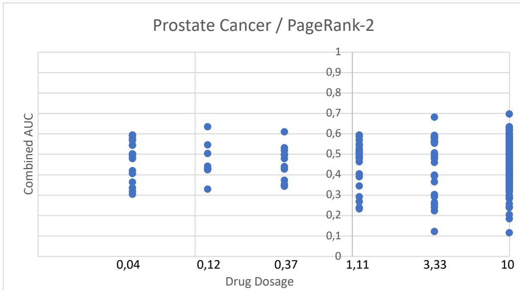
e) Distribution of AUC values with corresponding drug dosages in prostate cancer (using PageRank-2)
