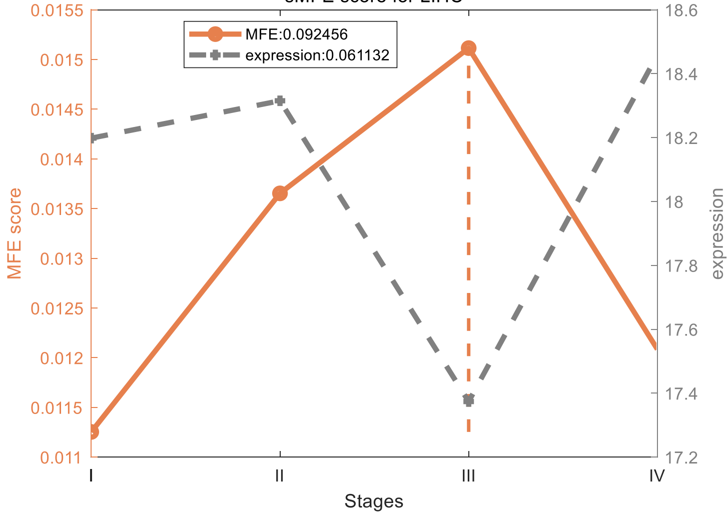
sMFE score for LIHC
