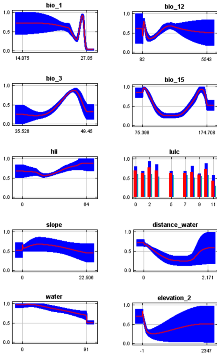
Figure S3. Showing the response curves of the all the final selected variable (n=50) iteration. Curves show how each environmental variable affects the Maxent prediction. The curves show how the predicted probability of presence changes as each environmental variable is varied, keeping all other environmental variables at their average sample value. The curves show the mean response of the 50 replicate Maxent runs (red) and and the mean \pm one standard deviation (blue, two shades for categorical variables).
