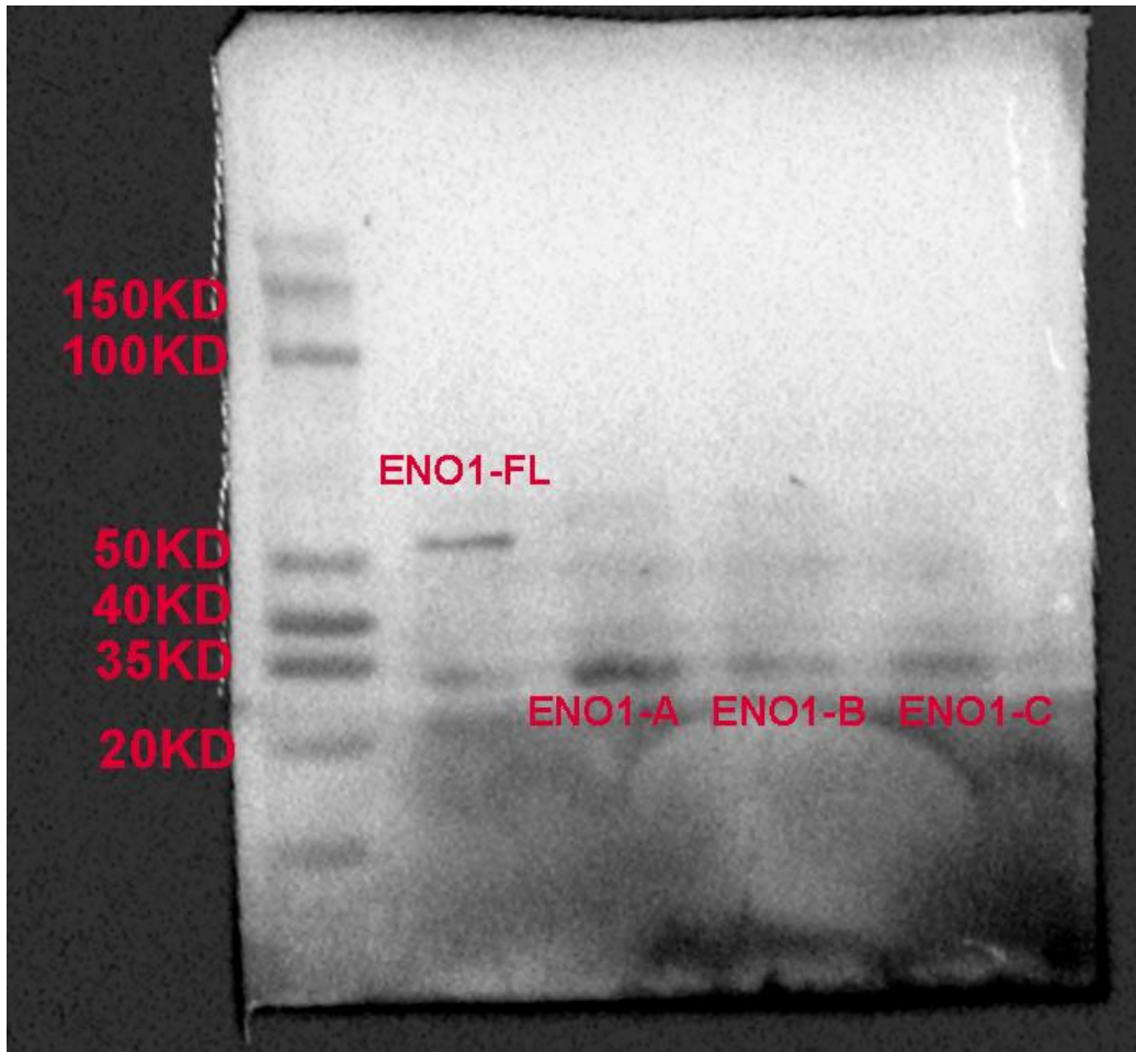
Supplementary Figure S1: Verifying ENO1 truncation efficiency by western blot
