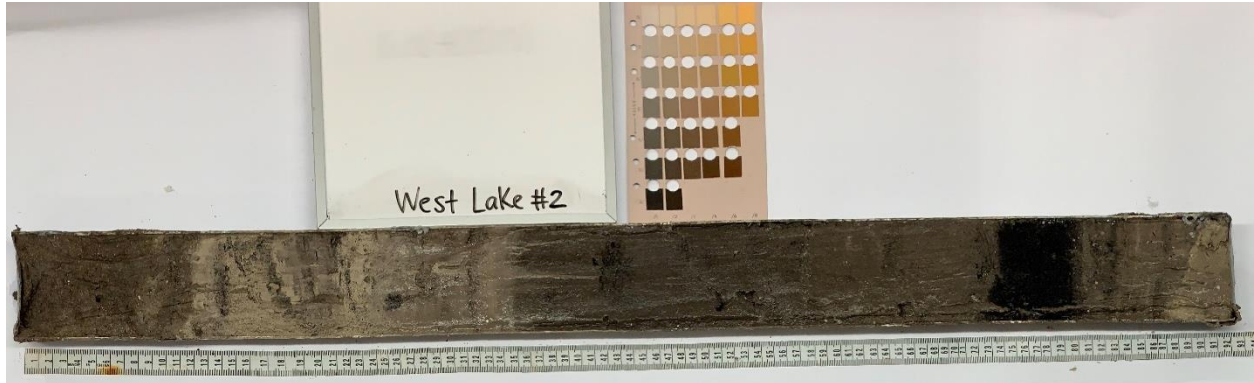
Figure S1. Split sediment cores for Dania Cutoff Canal (DCC), Park Education Center (PEC), Park Headquarters (PHQ), South Turning Basin (STB), and West Lake (WL). The left side of the core at 0 cm is the top (surface). Munsell sediment color chart is also shown.
